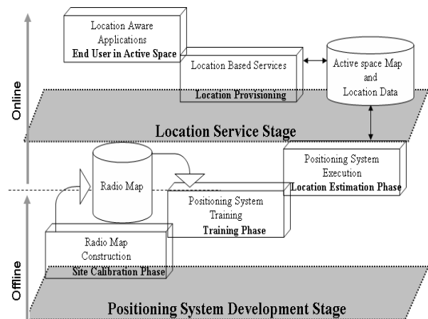
Fig. 3. Location System Development Life Cycle: Previous Approaches
