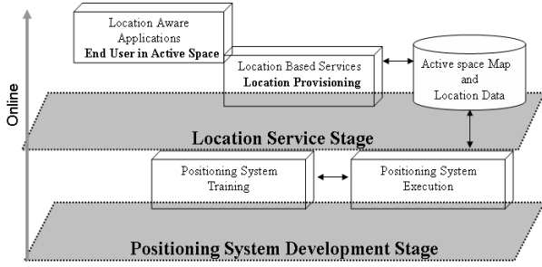
Fig. 4. Our Approach: Short Development Life Cycle
