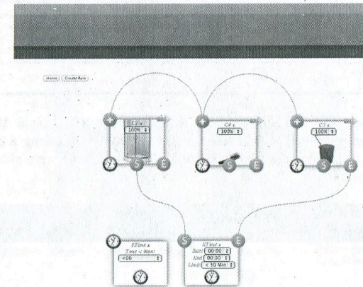
Fig. 3. Example of workspace and how objects selected from room view may be connected together.
