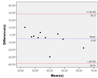
Figure 4: Agreement analysis between traditional TEA and mDurance through Bland-Altman plots. The mean of differences ( \bar{x} ) is represented by a blue line, while the limits of agreement ( \bar{x} \pm 1.96\sigma_X ) are depicted in red.
