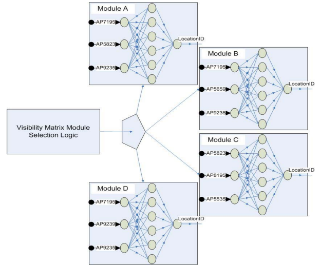
Fig 3: Modular Multi Layer Perceptron (MMLP) Architecture
