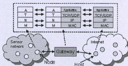
Fig. 1. Application-level Gateway
