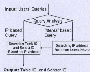
Fig. 15. Query Process
