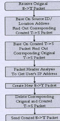
Fig. 8. Translation workflow of S->T
