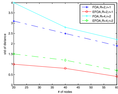
Fig. 12. Standard deviation of distance traveled versus number of nodes
