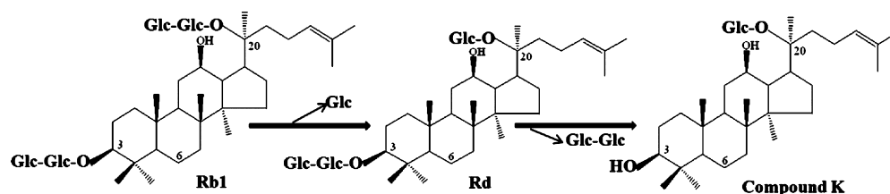
Figure 8. Transformation pathway from ginsenoside Rb1 to ginsenoside Rd and compound K by Bgp3.
