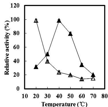
Figure 4. Effect of temperature on the stability and activity of recombinant Bgp3 determined using pNP- \beta -D-glucopyranoside as a substrate. \blacktriangle , the thermodependence of enzyme activity was assayed in 20 mM sodium phosphate buffer (pH 7.0) at various temperatures ranging from 20 to 70 °C. Maximum activity observed at 40 °C was taken as 100% = 29.4 U (mg protein) -1 . \triangle , thermostability was tested by incubating aliquots of the enzyme in 20 mM sodium phosphate buffer (pH 7.0) for 4 h at different temperatures.
