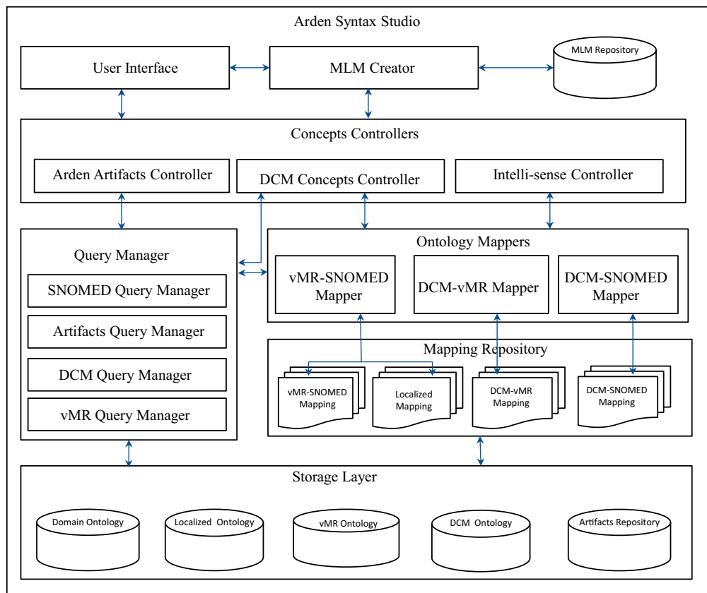
Fig. 2. I-KAT architecture.
